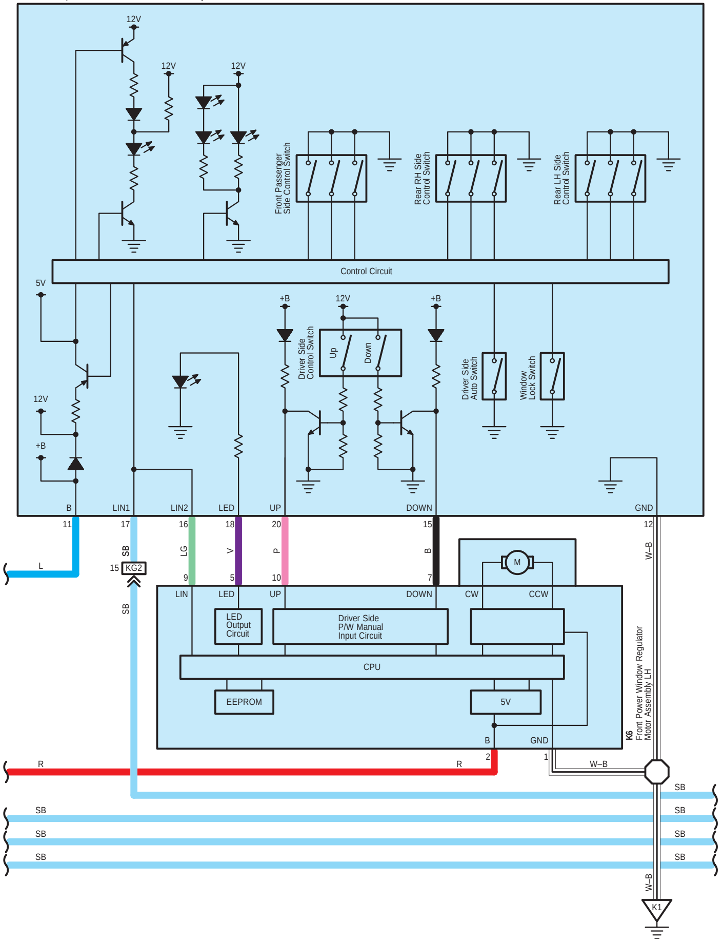
K3 Multiplex Network Master Switch Assembly
